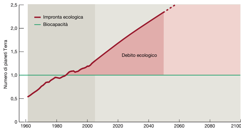
Fig. 31: SCENARIO BAU (BUSINESS AS USUAL) E DEBITO ECOLOGICO
